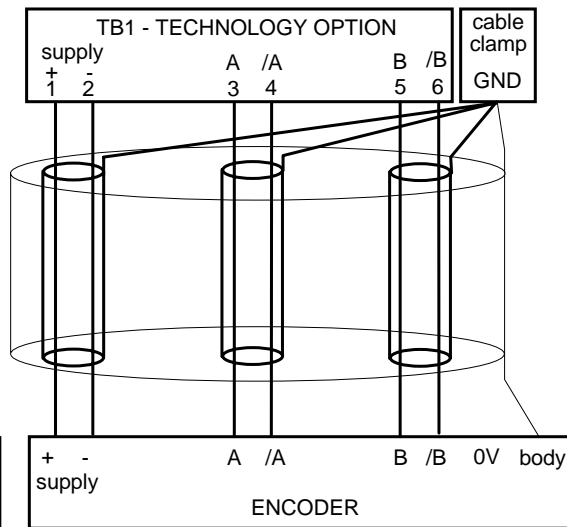
Figure 2 Differential Encoder Outputs
