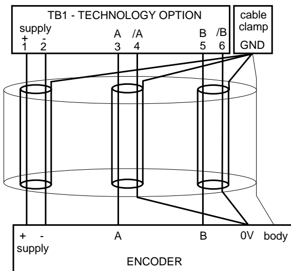
Figure 3 Single-Ended Encoder Outputs
