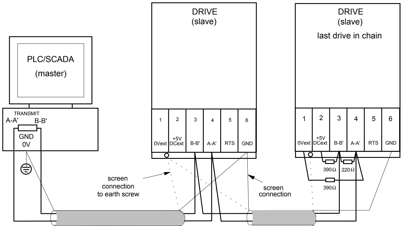
Figure 5 Typical Wiring Diagram
